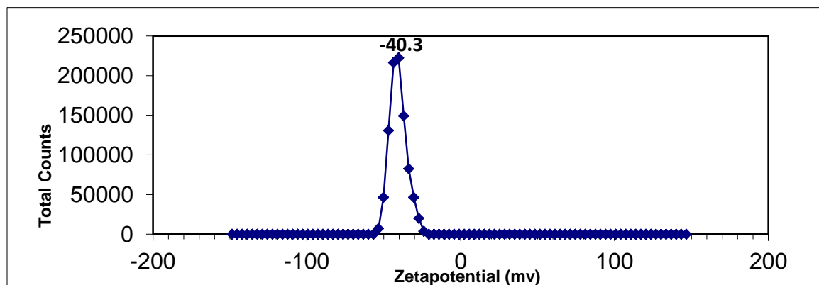
Figure 4.11. Zeta potential measurements for froth of dispersant only
