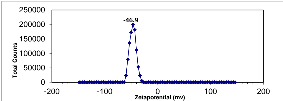
Figure 4.12. Zeta potential measurements for froth of PAM
